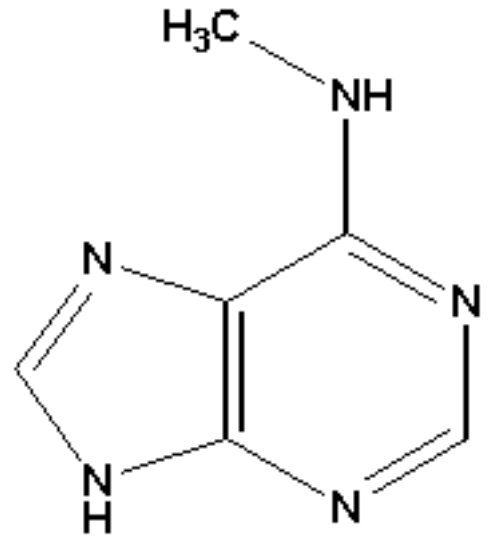
N6-methyladenine (mA)
