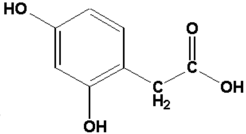
Homogentisic Acid
