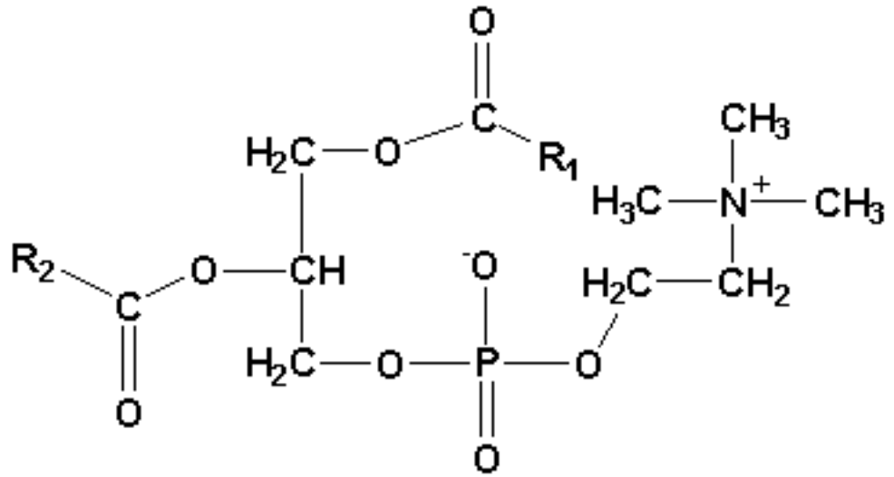
Phosphatidylcholine
