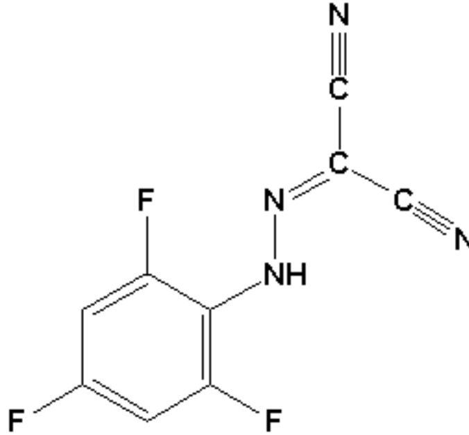
Trifluorocarbonylcyanide phenylhydrazine
