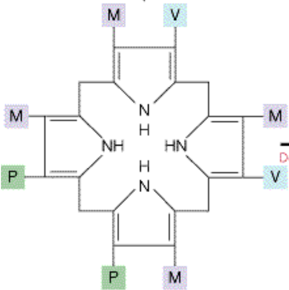
Protoporphyrinogen IX
