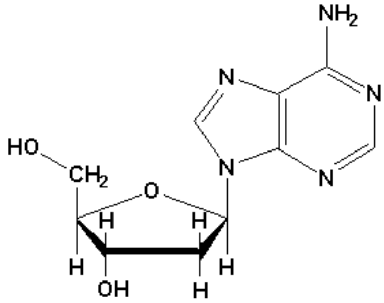
Deoxyadenosine
