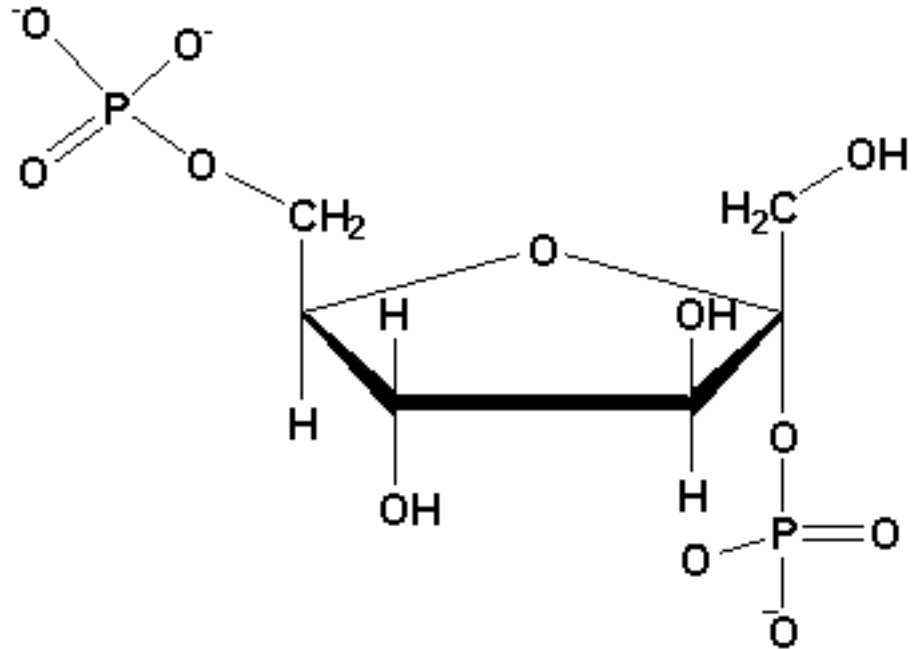
Fructose-2,6-bisphosphate
