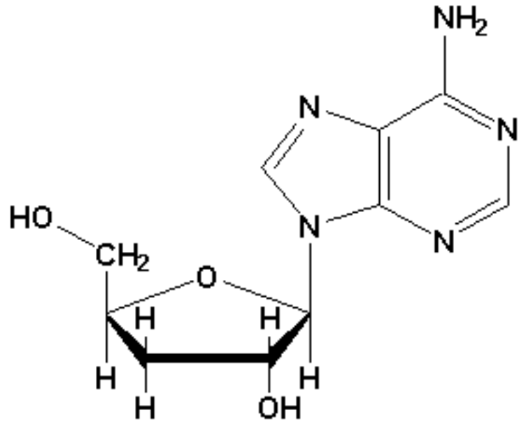
Cordycepin (3'-deoxyadenosine)
