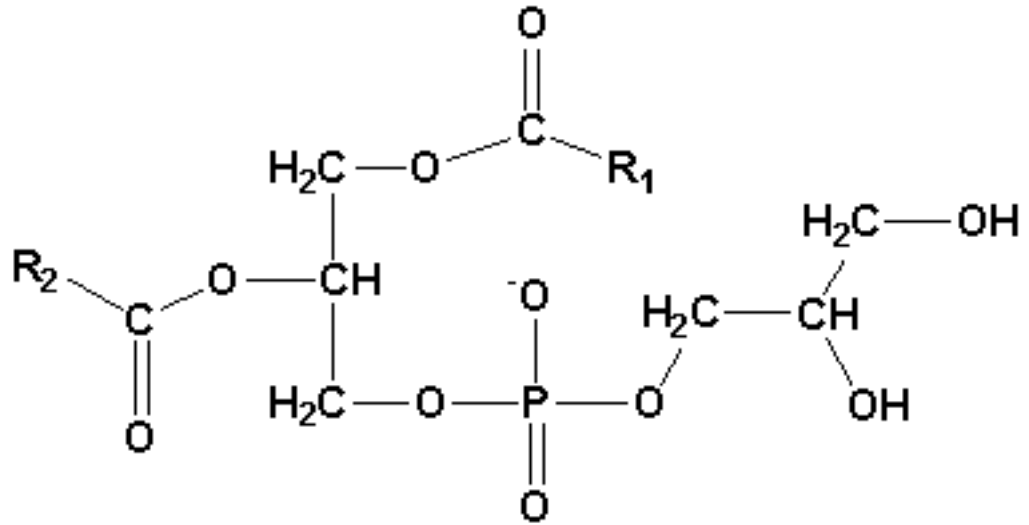
Phosphatidylglycerol
