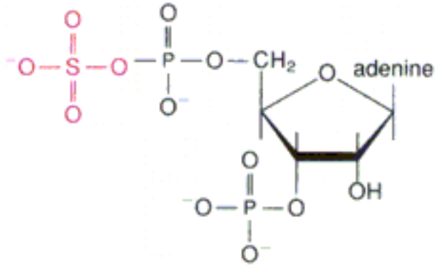
3'-Phosphoadenosine-5'-phosphosulfate
