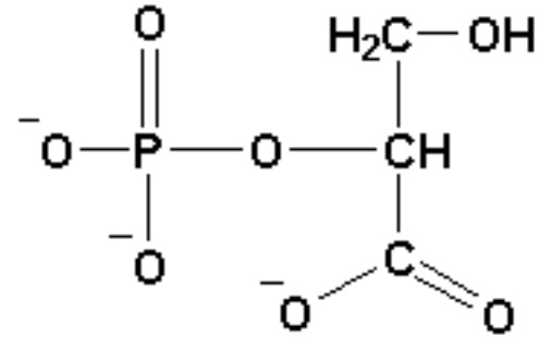
2-Phosphoglycerate
