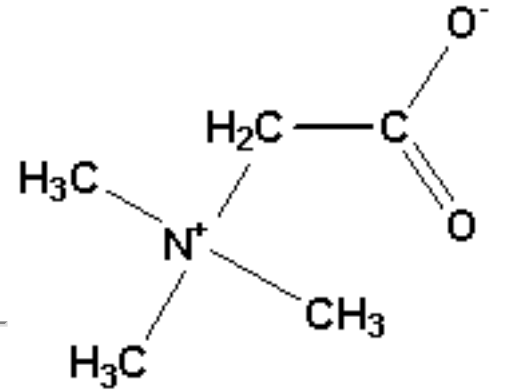
Glycine Betaine
