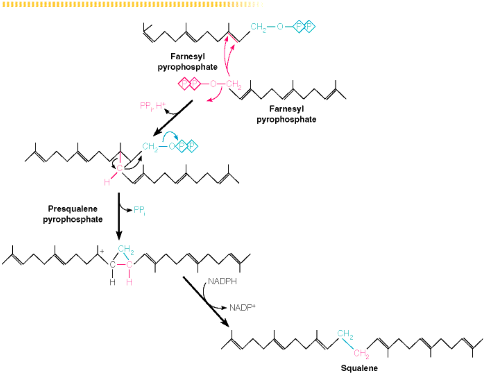
Figure 19.21: Conversion of farnesyl pyrophosphate to squalene.
