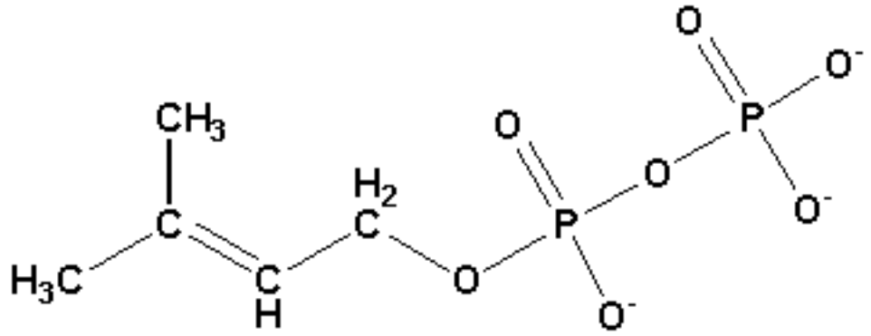
Dimethylallyl Pyrophosphate
