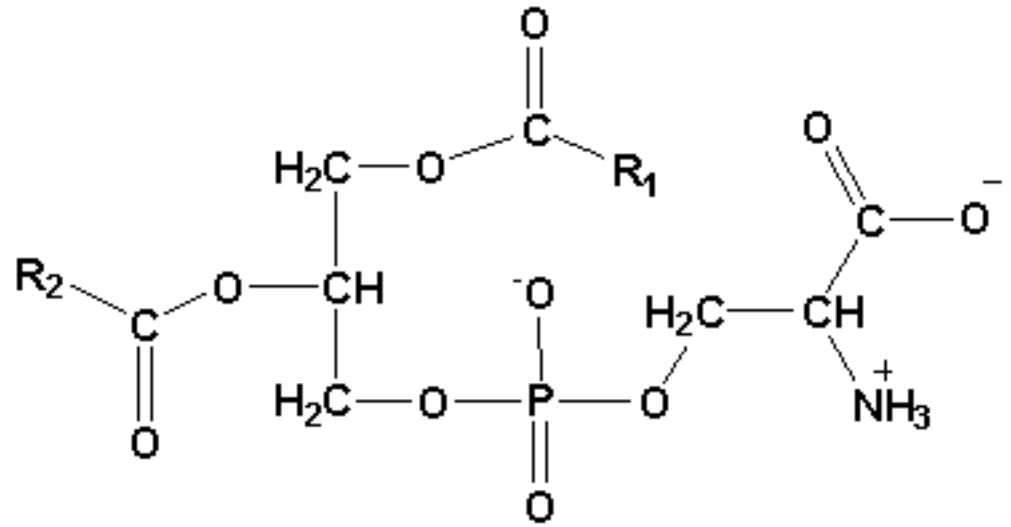
Phosphatidylserine
