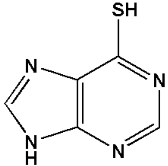
6-Mercaptopurine
