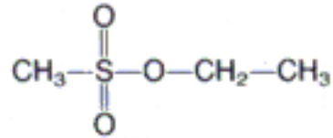
Ethylmethanesulfonate (EMS)
