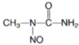
Methylnitrosourea (MNU)
