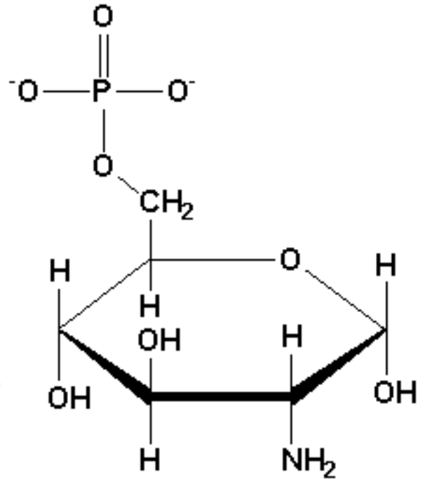
Glucosamine-6-phosphate
