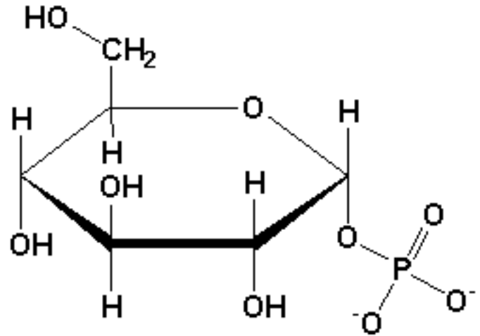
Glucose-1-phosphate
