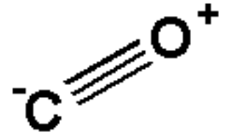
Carbon Monoxide
