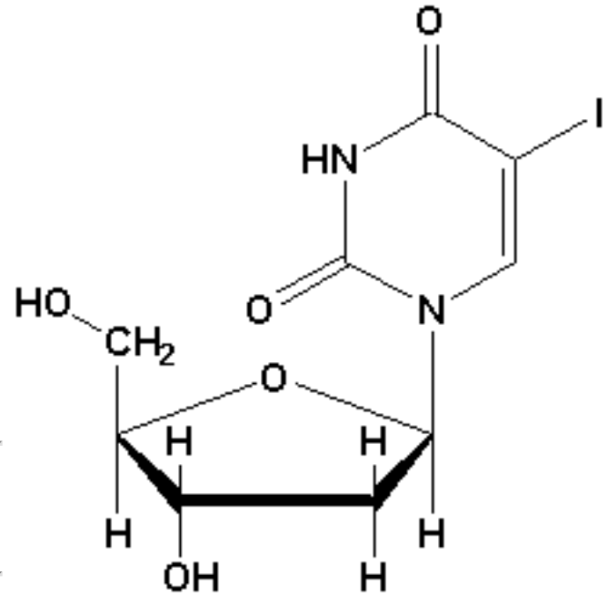
5-Iododeoxyuridine
