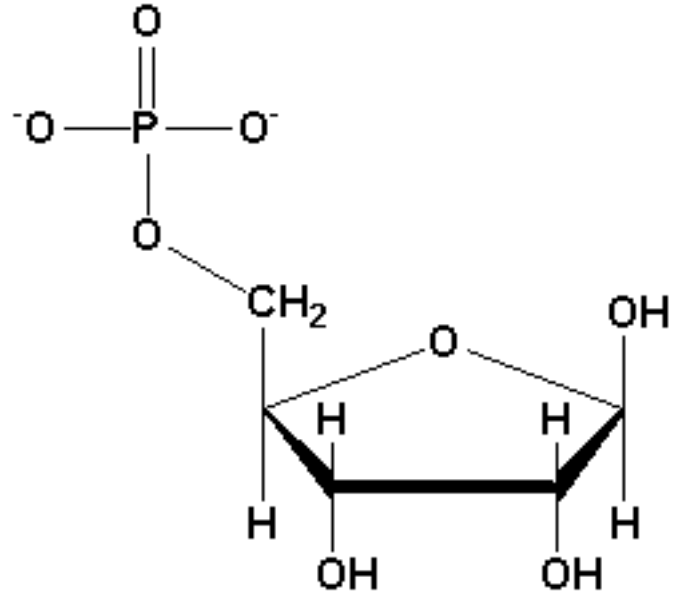
D-Ribose-5-phosphate
