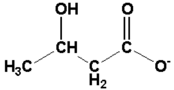
beta-hydroxybutyrate
