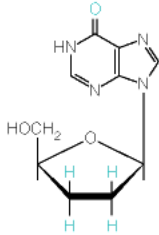
2',3'-Dideoxyinosine
