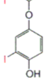
Triiodothyronine (T 3 )
