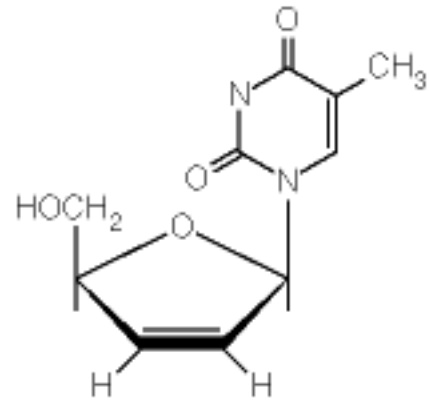
2',3'-Didehydro-3'-deoxythymidine
