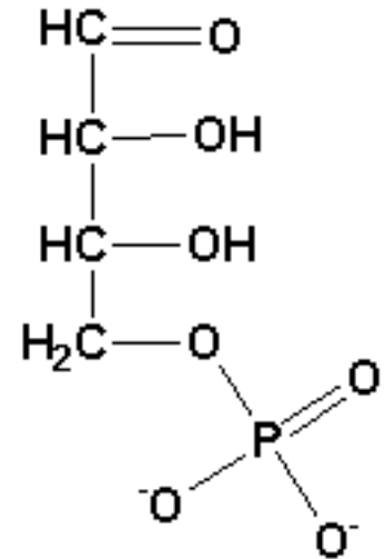
Erythrose-4-phosphate
