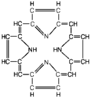
(a) Porphin (C 20 H 14 N 4 )
