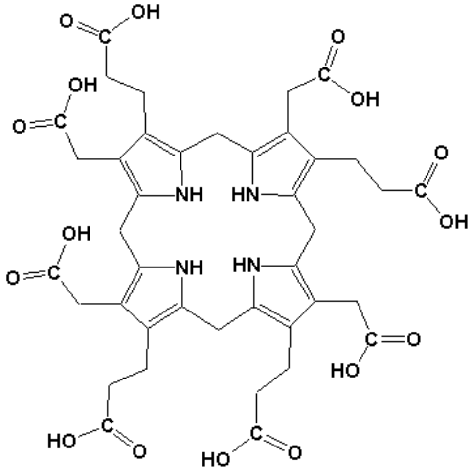
Uroporphyrinogen III
