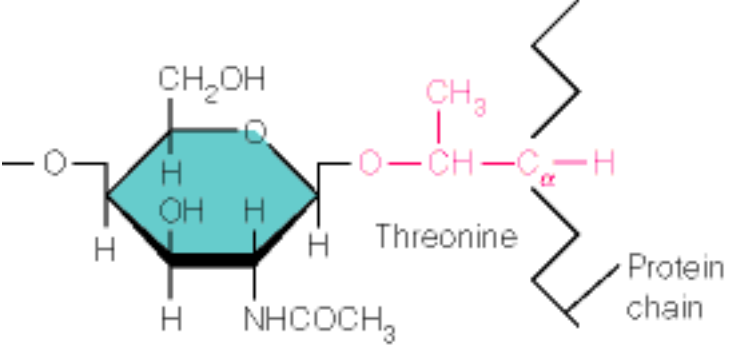
(b) N-Acetylgalactosamine
