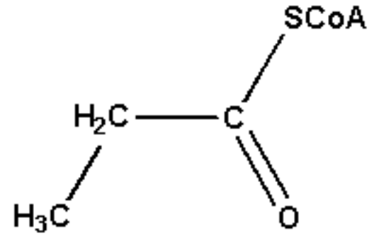
Propionyl-CoA
