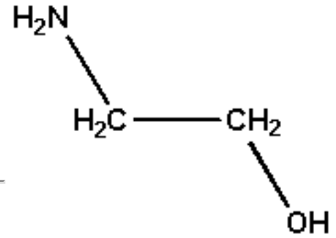
Ethanolamine
