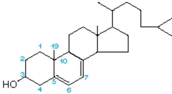
7-Dehydrocholesterol
