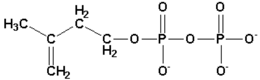
Isopentenyl Pyrophosphate
