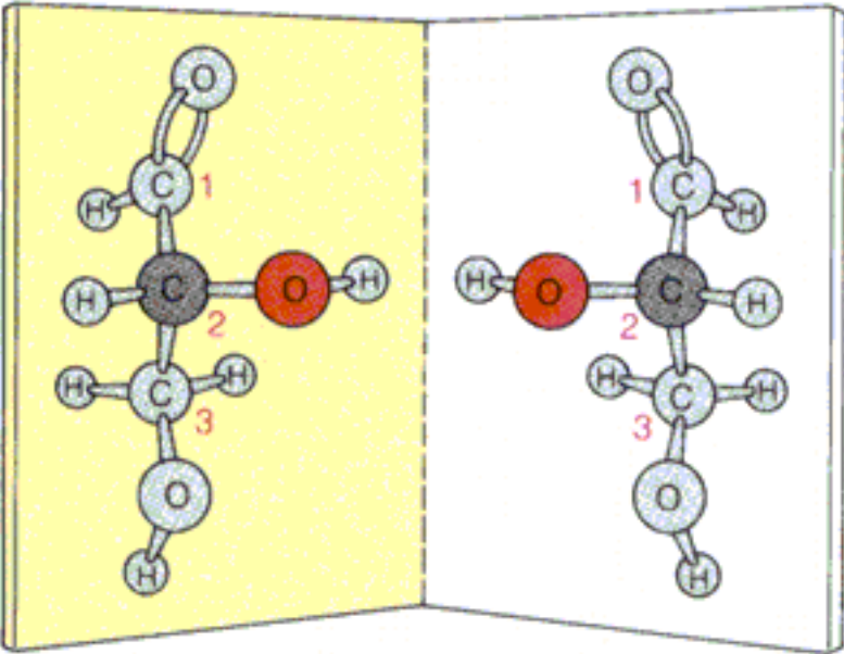
D-Glyceraldehyde
