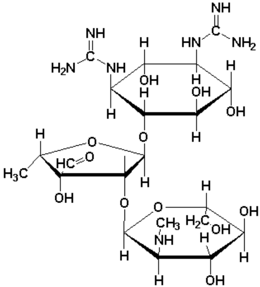
Streptomycin
