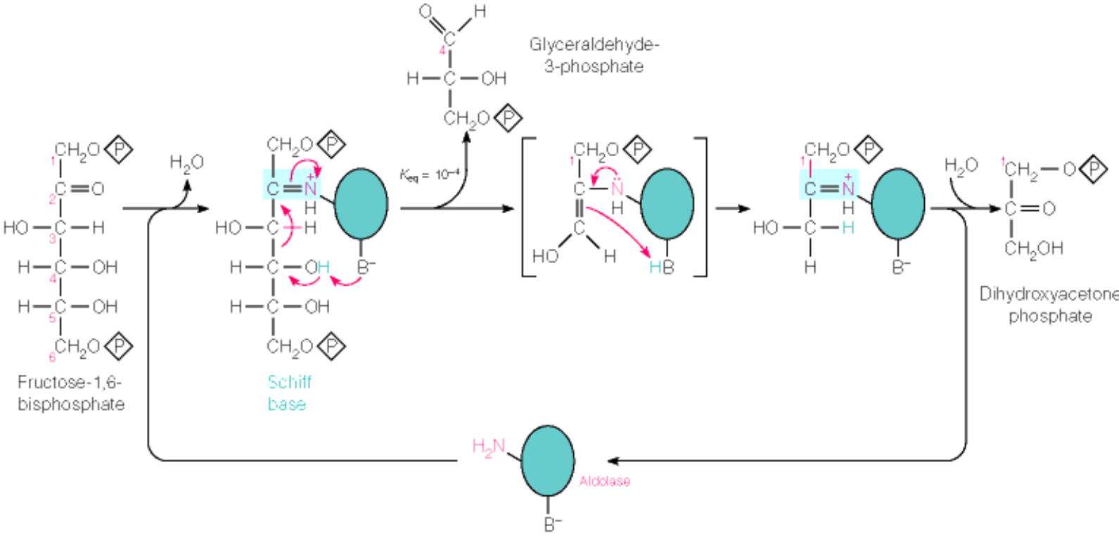
Figure 13.4: Reaction mechanism for fructose-1,6-bisphosphate aldolase.
