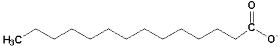
Myristate
