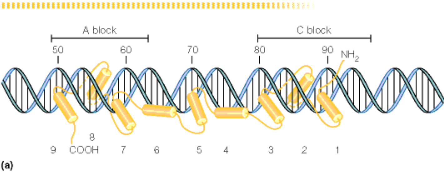
Figure 28.22: Zinc fingers.
