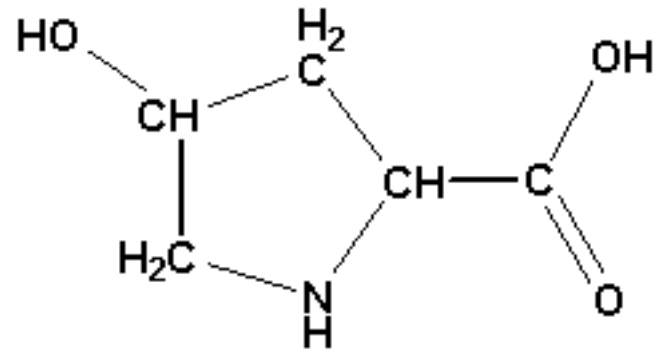
Hydroxyproline
