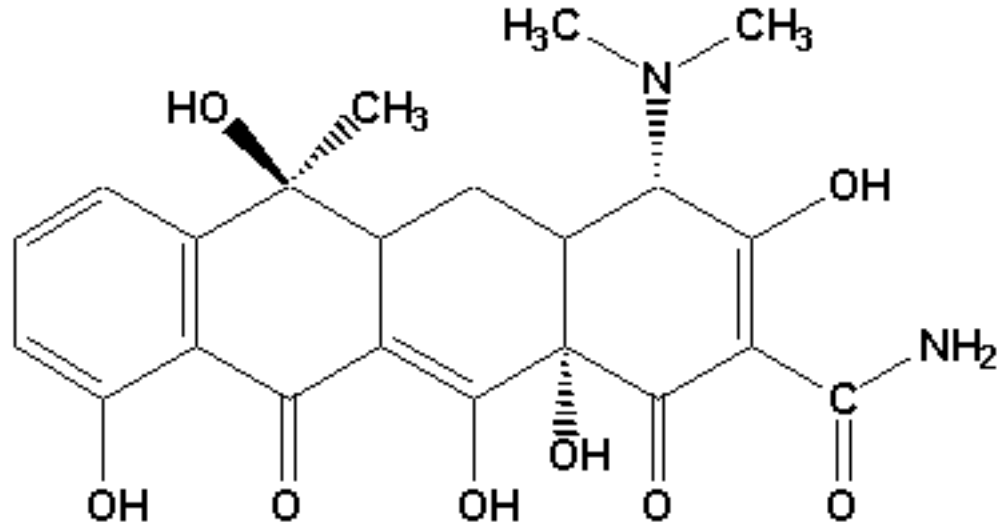
Tetracycline
