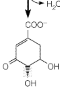
3-Dehydroshikimate
