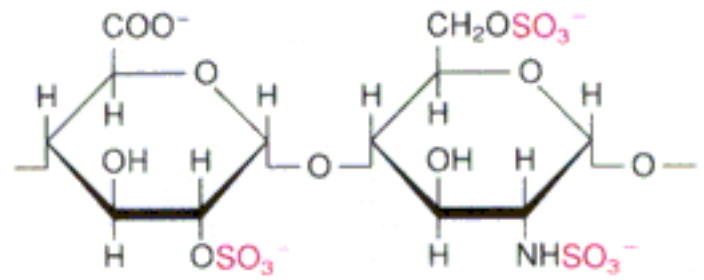
Heparin
