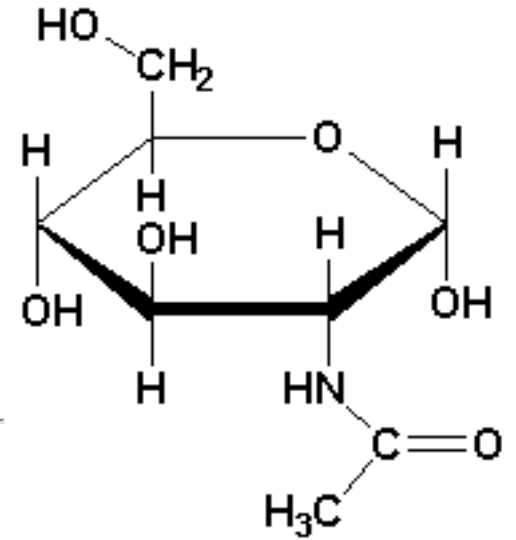
N-acetylglucosamine
