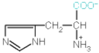
Histidine
