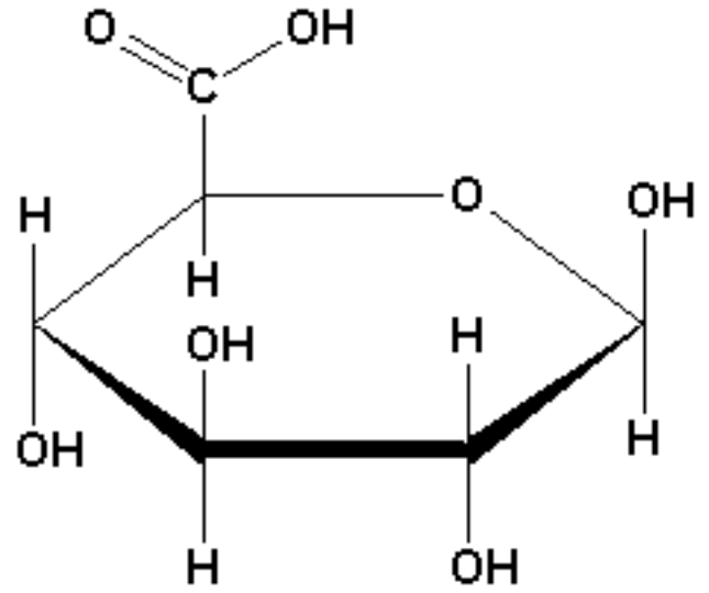
Glucuronic Acid
