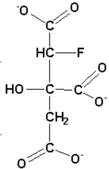
Fluorocitrate
