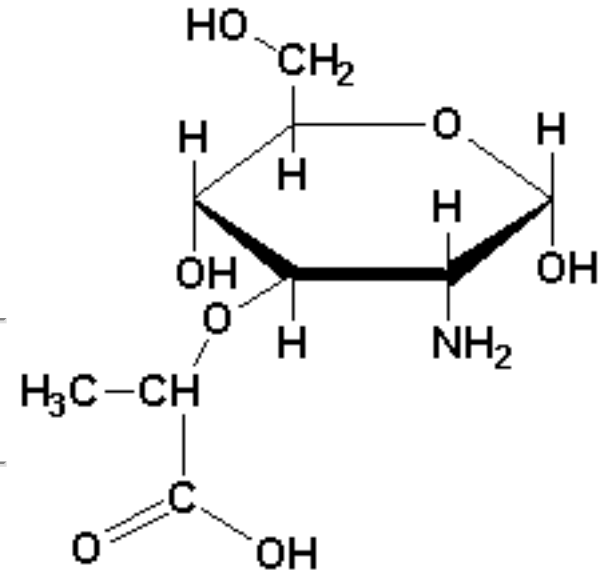
Muramic Acid
