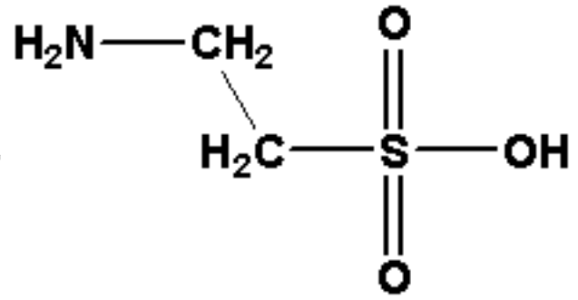
Taurine
