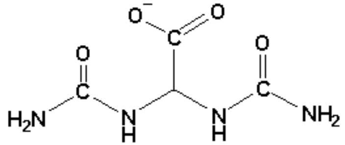
Allantoic Acid
