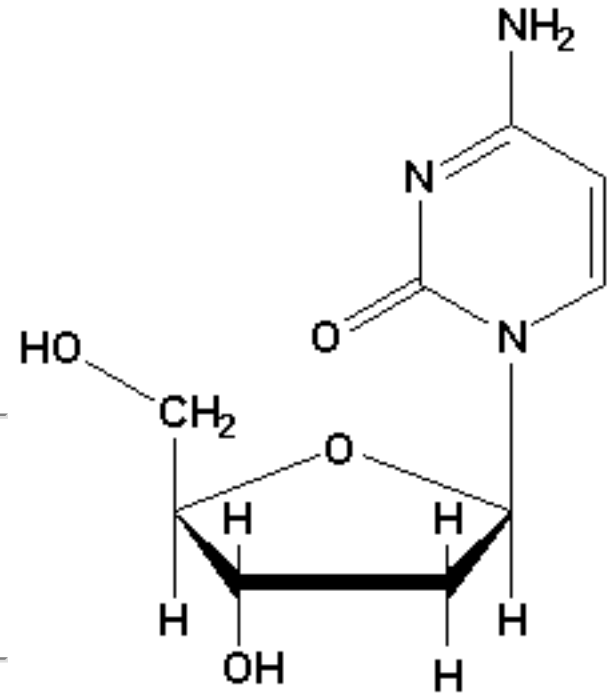
Deoxycytidine
