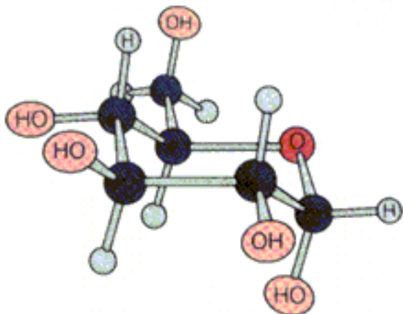
Chair
