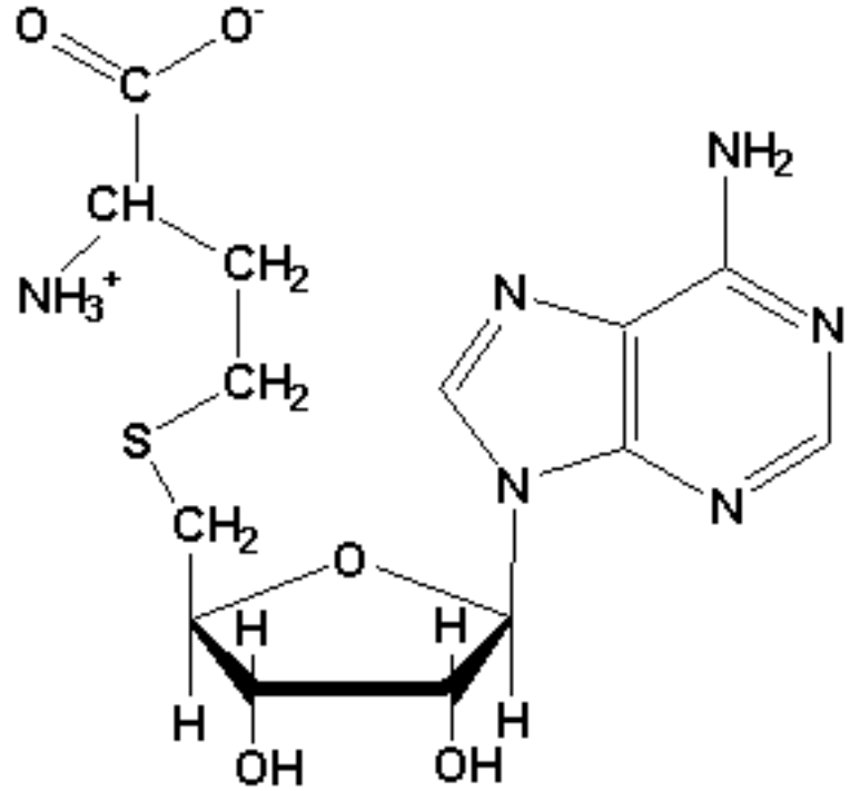
S-Adenosylhomocysteine
