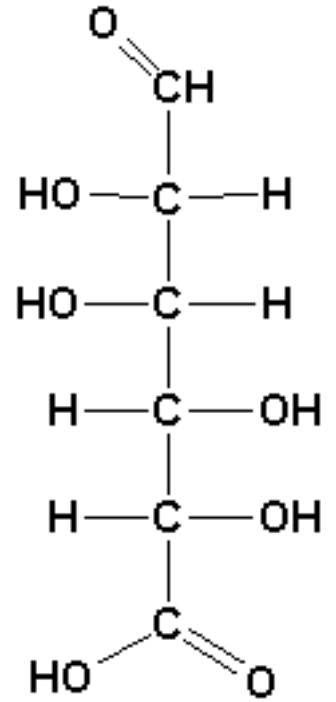
Mannuronic Acid
