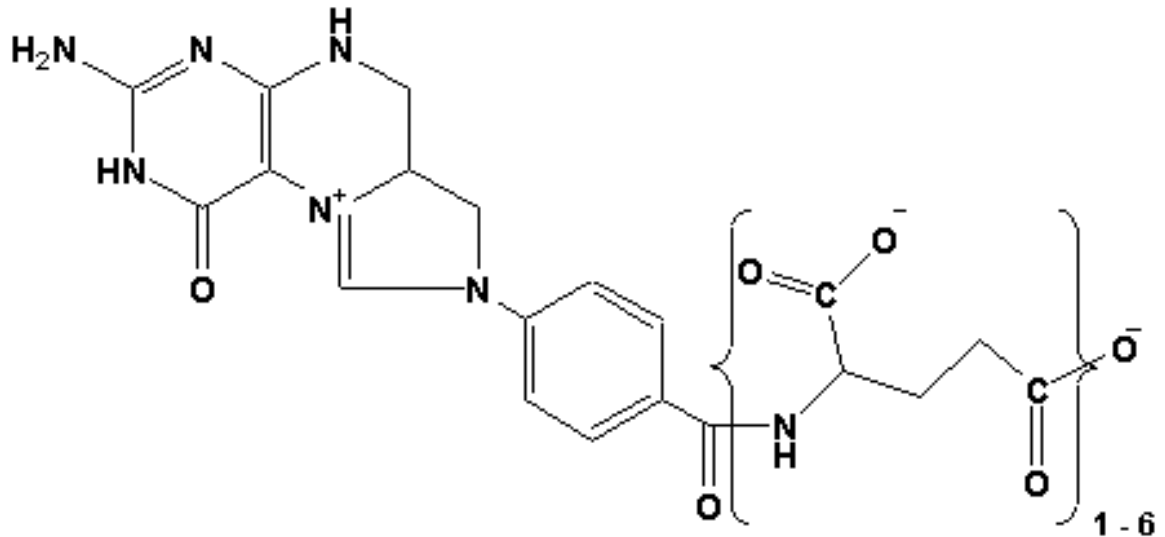
5,10-Methenyltetrahydrofolate
