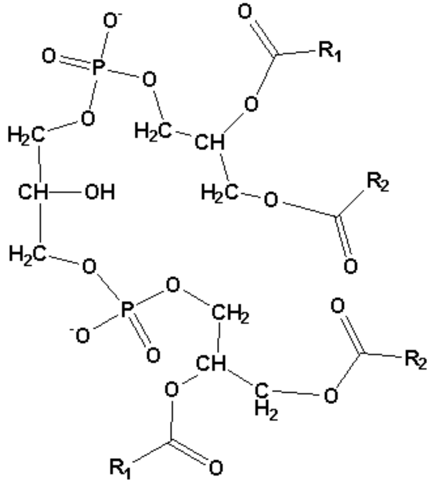
Cardiolipin
