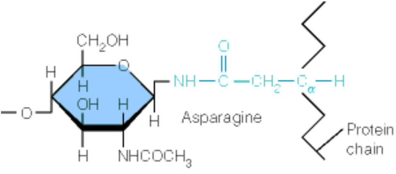
(a) N-Acetylglucosamine
