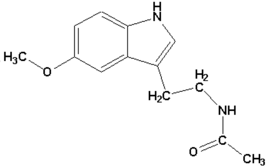
Melatonin (O-methyl-N-acetylserotonin)
