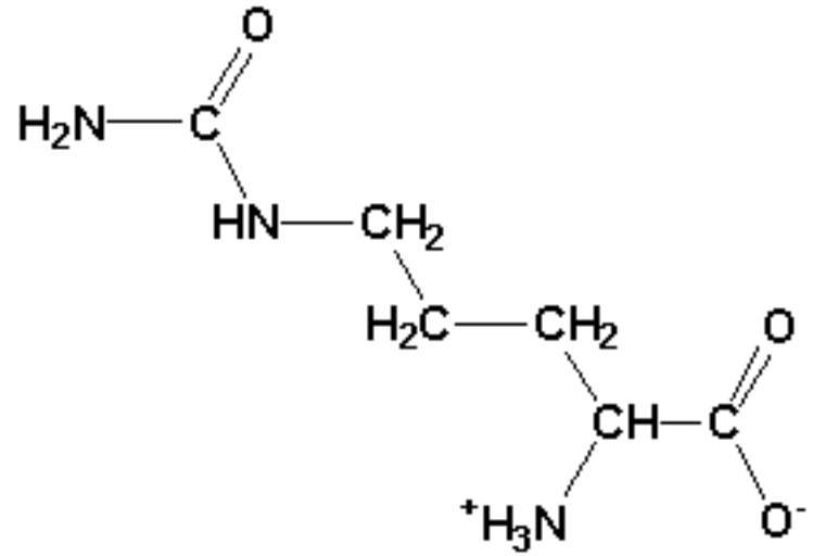
Citrulline
