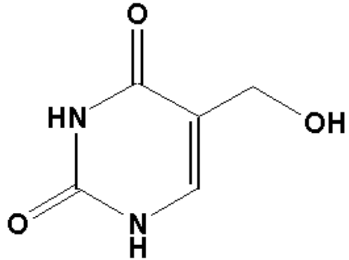
5-Hydroxymethyluracil
