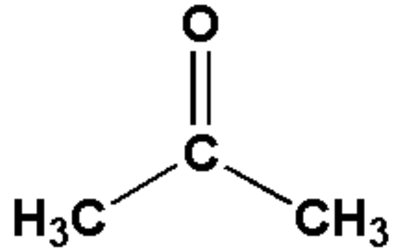
Acetone
