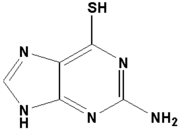
6-Thioguanine
