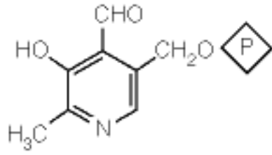
Pyridoxal phosphate
