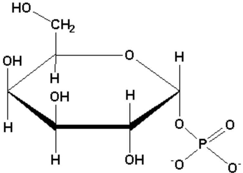
Galactose-1-phosphate
