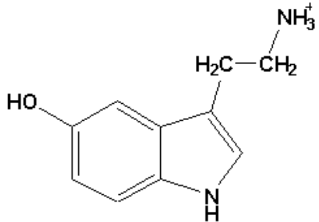
Serotonin (5-hydroxytryptamine)
