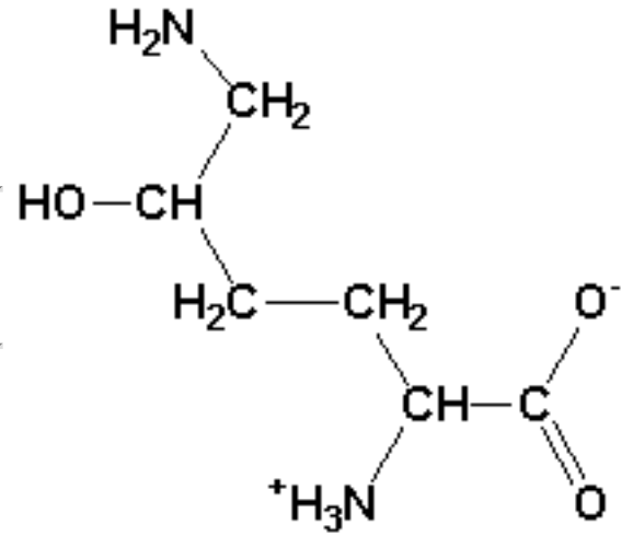
Hydroxylysine
