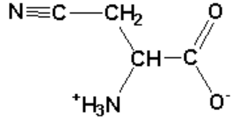
Beta-cyanoalanine
