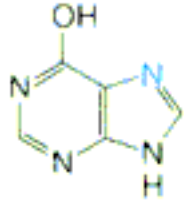
Hypoxanthine
