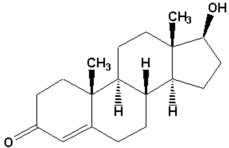
Testosterone
