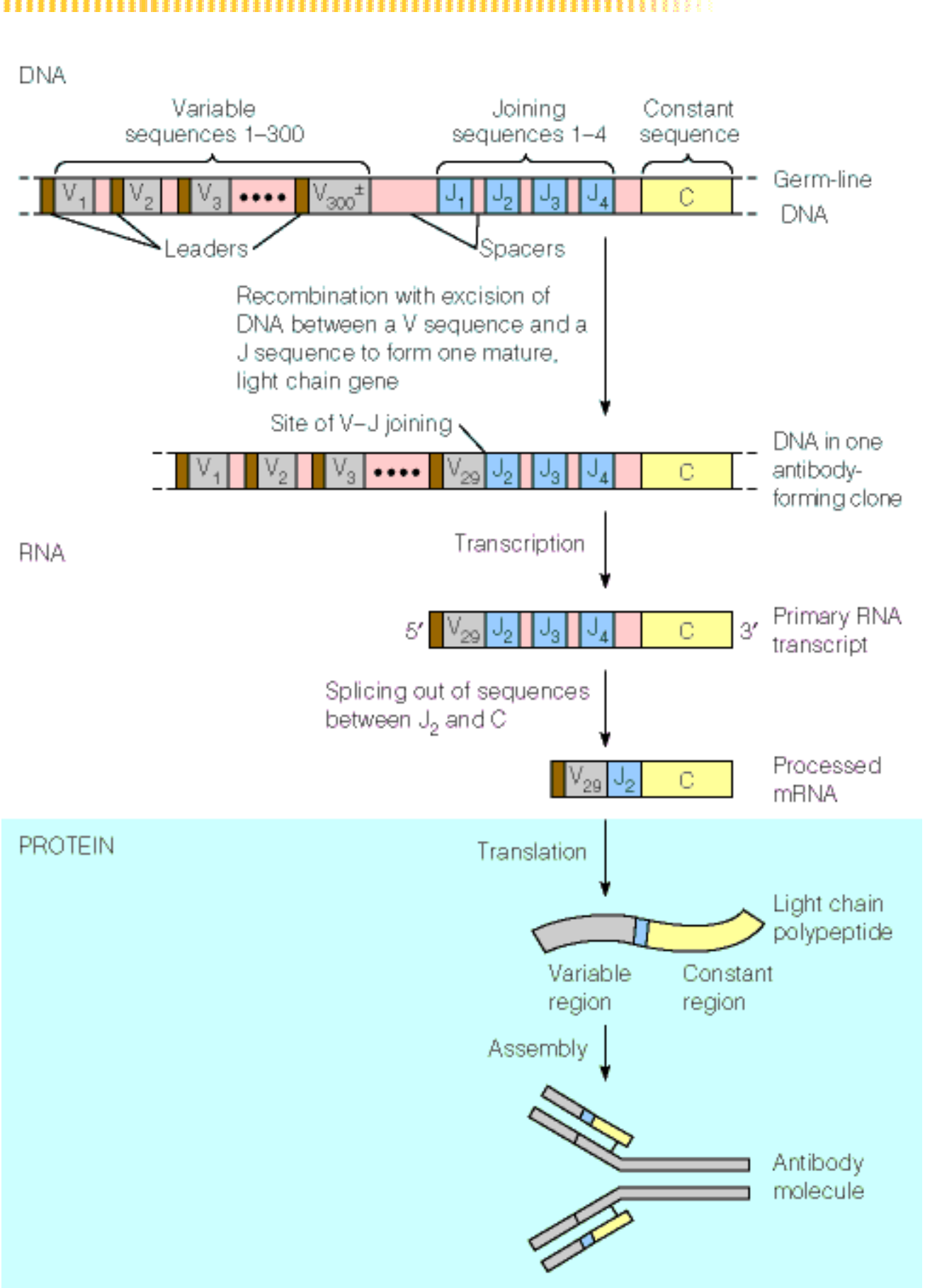
Figure 25.32: Gene rearrangements in antibody gene maturation.
