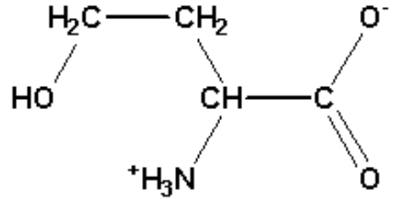
Homoserine
