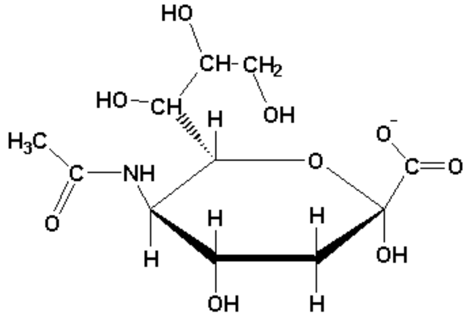
N-Acetyl-Neuraminic Acid
