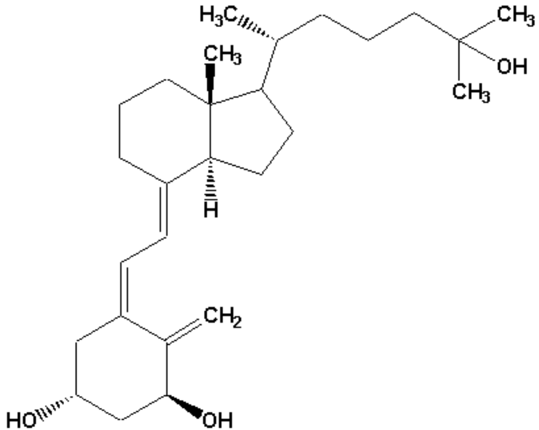
1,25-Dihydroxycholecalciferol
