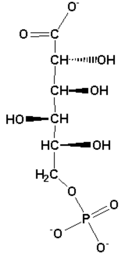
6-phosphogluconate
