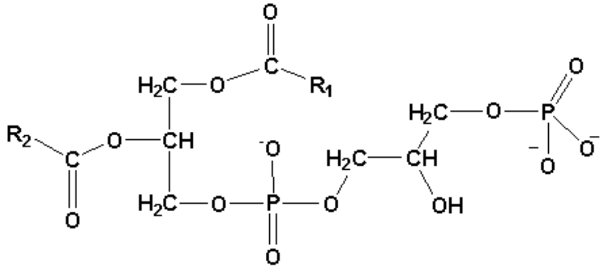
Phosphatidylglycerol-3-phosphate
