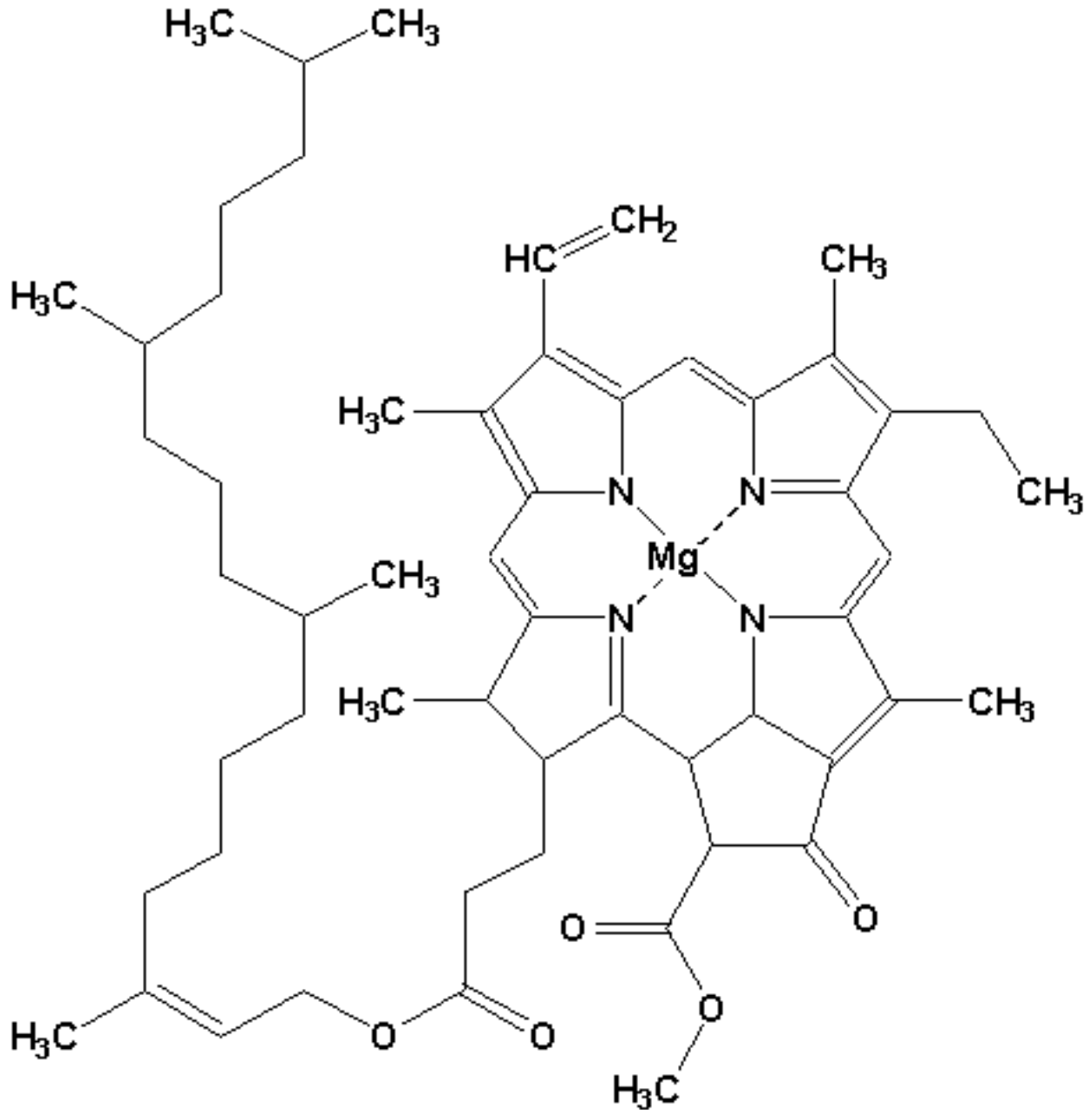
Chlorophyll A
