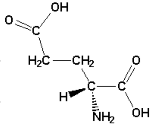
D-glutamic acid
