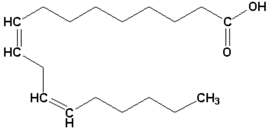
Linoleic Acid
