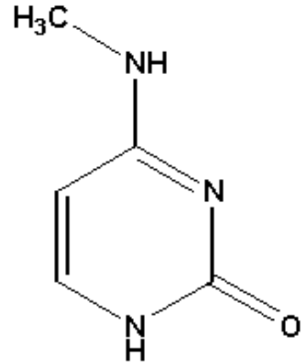
N4-methylcytosine
