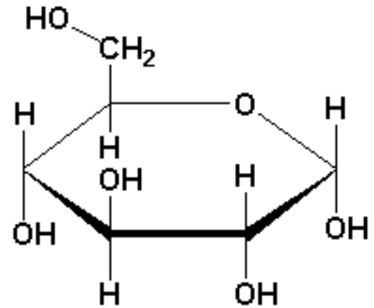
Glucose
