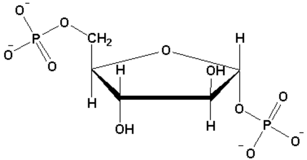
Ribulose-1,5-bisphosphate (RuBP)
