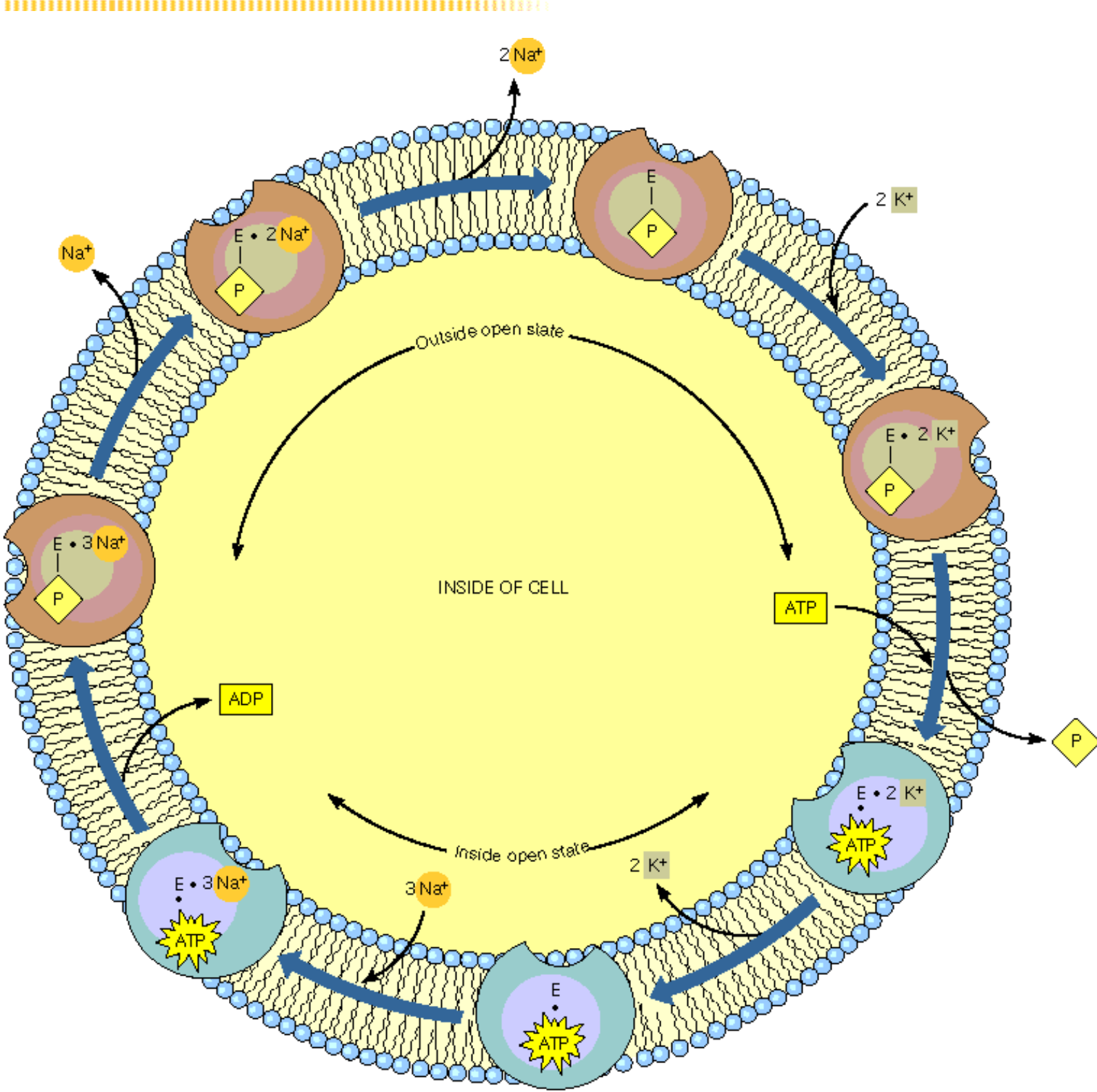
Figure 10.26: A schematic diagram of the functional cycle of the Na + -K + pump.
