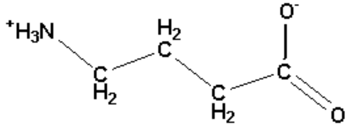
Gamma-aminobutyric acid
